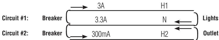
SureTest Shared Neutral Test w/300mA load
